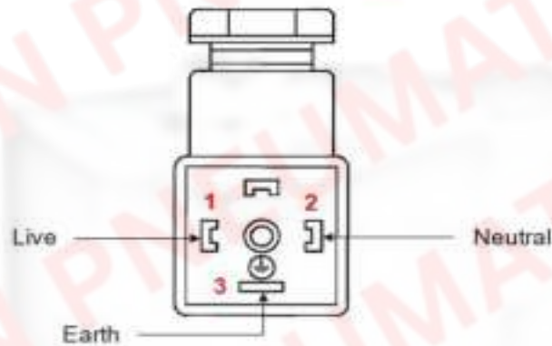
Wiring Connections AC
